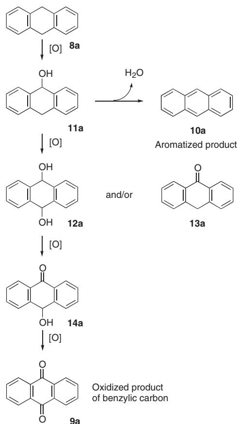
Fig. 2. Reaction pathway from 9,10-dihydroanthracene to anthraquinone and anthracene.
