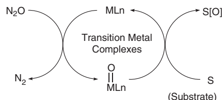
Fig. 1. Catalytic cycle of \text{N}_2\text{O} oxidation.
